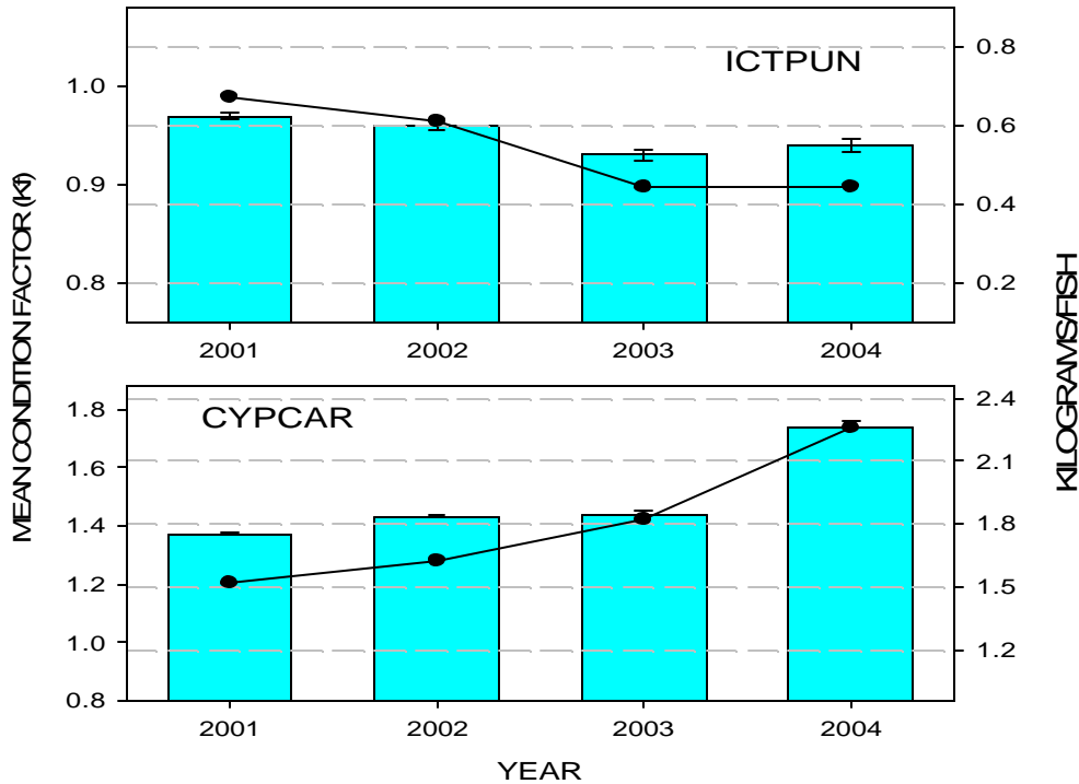
Figure 7. Mean condition factor K_{(t)} and kilograms/fish of channel catfish [ICTPUN] and common carp [CYPCAR] collected from PNM Weir to Hogback Diversion, 2001-2004. Bars represent Mean K_{(t)} and lines represent kilograms/fish.
