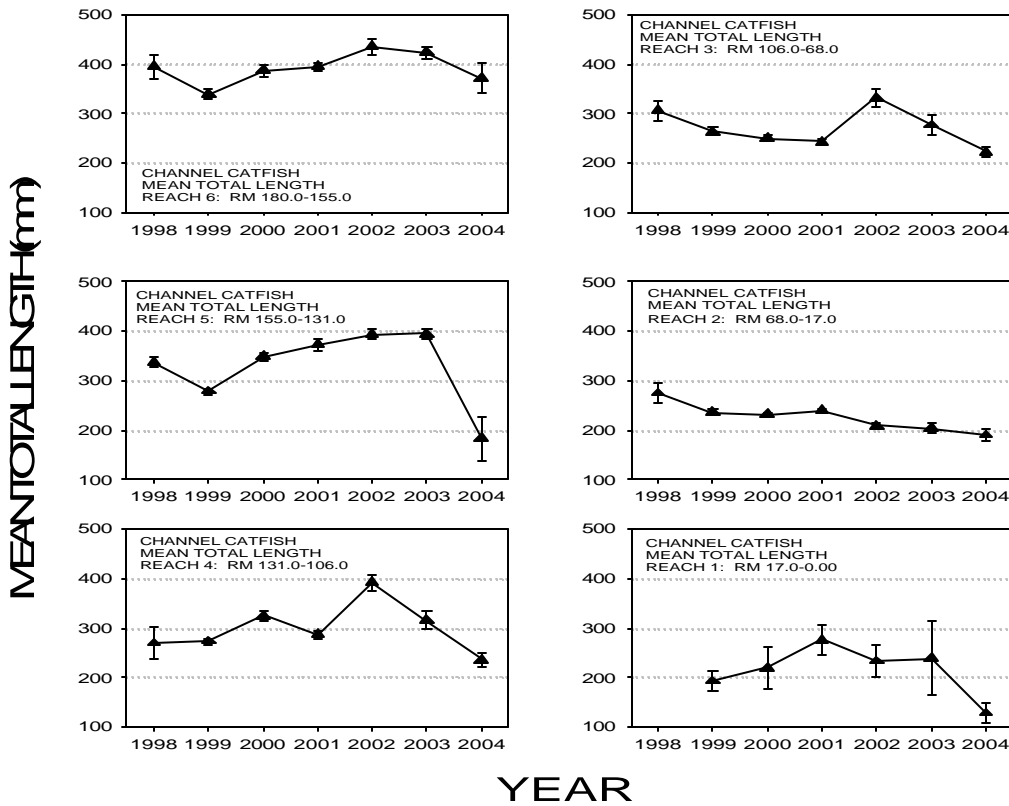
Figure 20. Mean total length (mm) of channel catfish by Geomorphic Reach and by year. Error bars represent \pm 1 SE.
