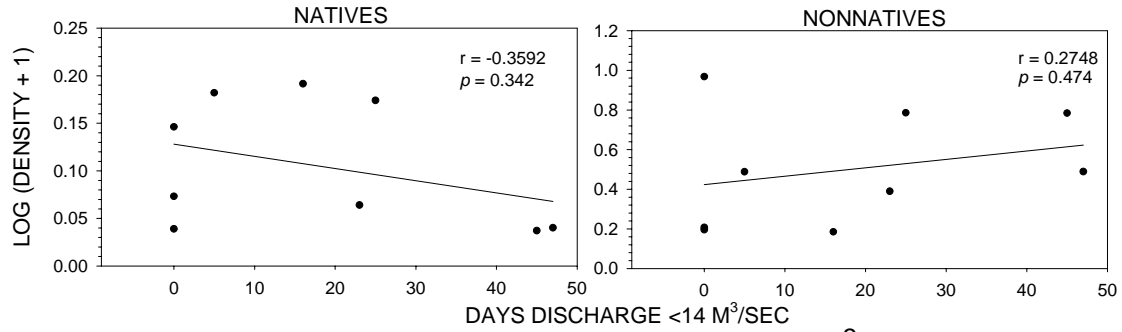
Figure 59. Number days mean daily summer discharge <14.0 m 3 /sec versus autumn density of native and nonnative fishes in San Juan River Reach 3 secondary channels, 1993 - 2001.
