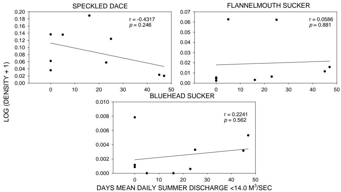
Figure 60. Number days mean daily summer discharge <14.0 m 3 /sec versus autumn density of native fish species density in San Juan River Reach 3 secondary channels, 1993 - 2001.
