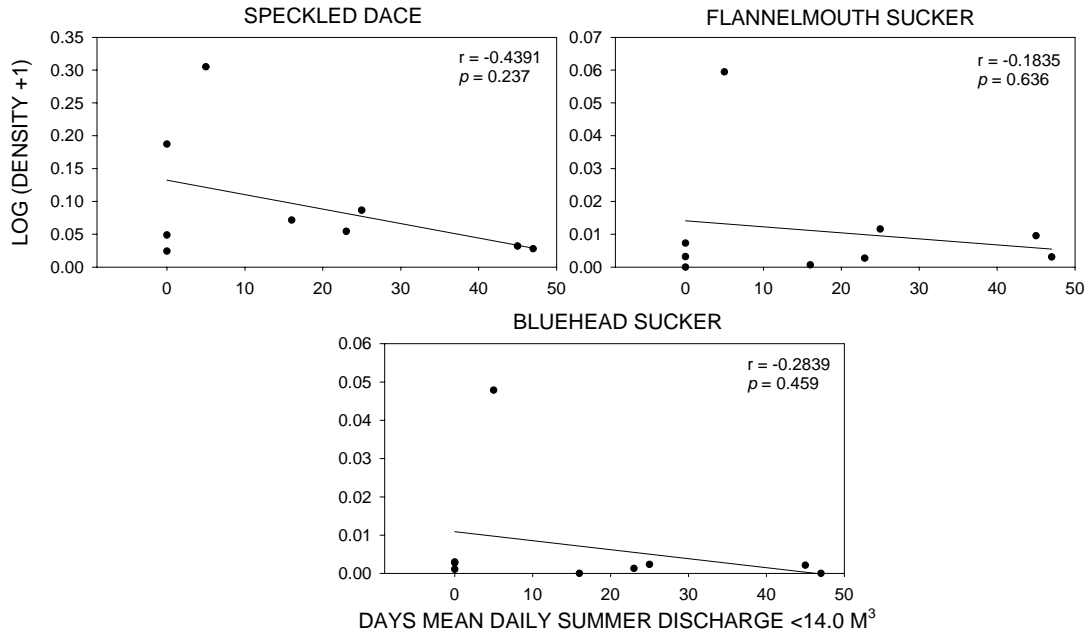
Figure 48. Number days mean daily summer discharge <14.0 m 3 /sec versus native fish densities in San Juan River Reach 4 secondary channels, 1993 - 2001.
