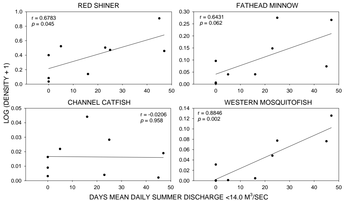
Figure 49. Number days mean daily summer discharge <14.0 m 3 /sec versus nonnative fish species density in San Juan River Reach 4 secondary channels, 1993 - 2001.
