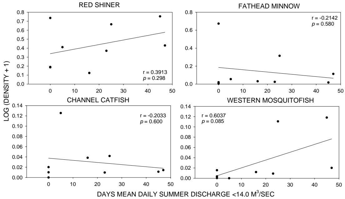
Figure 61. Number days mean daily summer discharge <math><14.0\text{ m}^3/\text{sec}</math> versus autumn nonnative fish species density in San Juan River Reach 3 secondary channels, 1993 - 2001.
