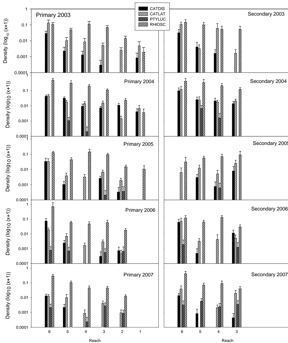
Figure 24. \text{Log}_{10}(x+1) density of commonly collected native species and Colorado pikeminnow in the San Juan River, by reach, from 2003 through 2007.
