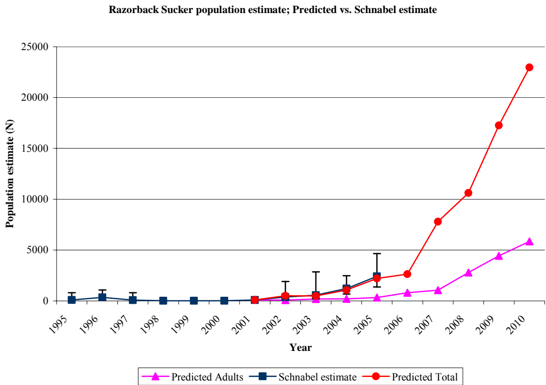
Figure 45. Comparison of monitored versus modeled razorback sucker populations.
