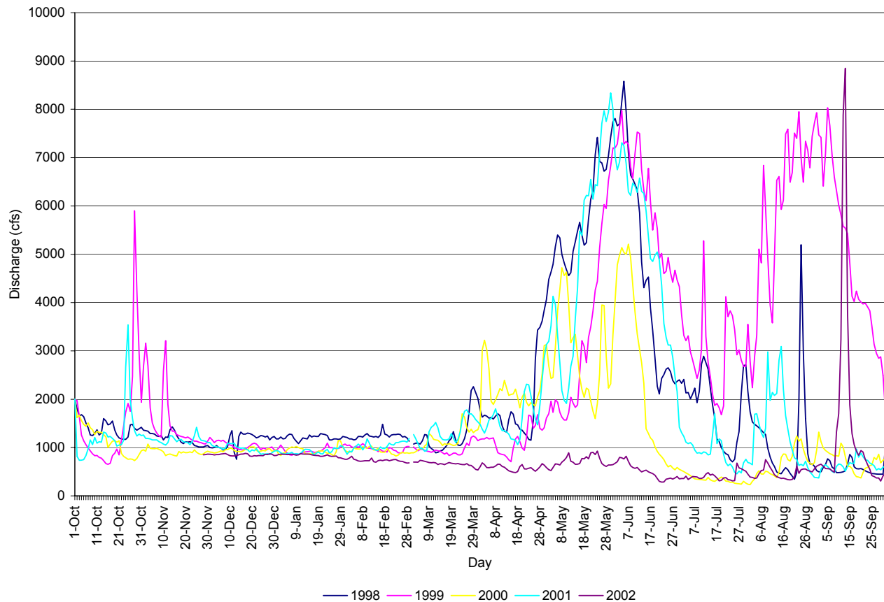
Figure 1. Average daily discharge at USGS gage# 09371010 near Four Corners, CO, from 1998-2002.
