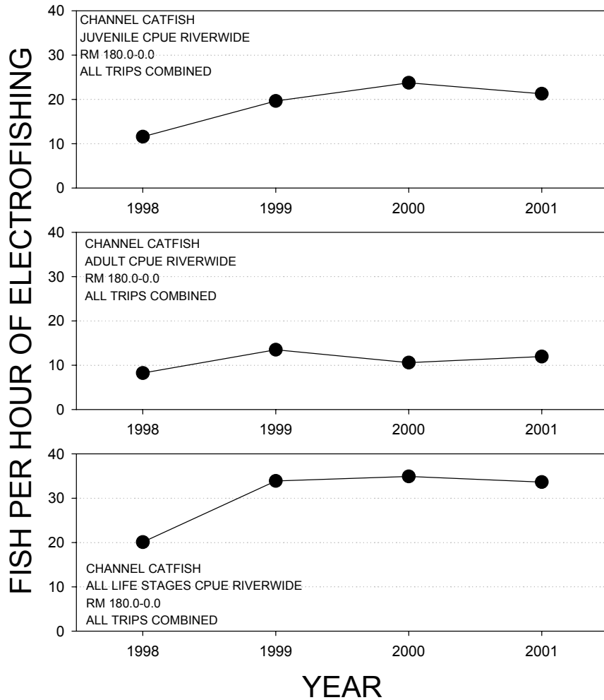
Figure 5. Riverwide CPUE for channel catfish removed during all sampling in the San Juan River from 1998-2001 (Davis 2003).
